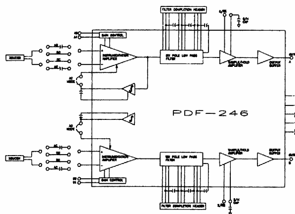
PDF-246 BLOCK AND TYPICAL CONNECTION DIAGRAM
